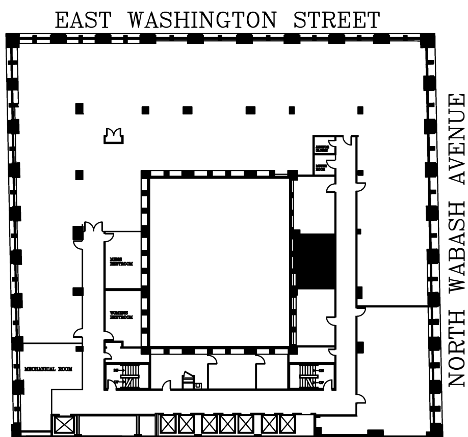
LEVEL 9 CONTEXT PLAN
